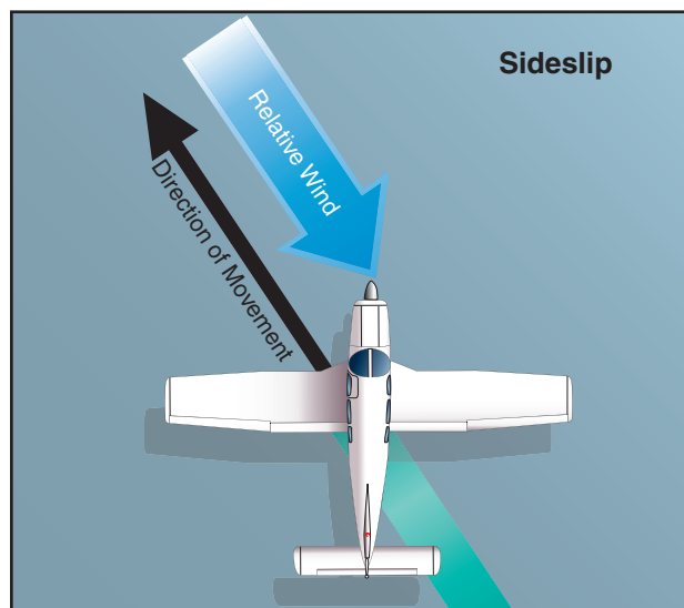
Figure 8-12. Sideslip.
